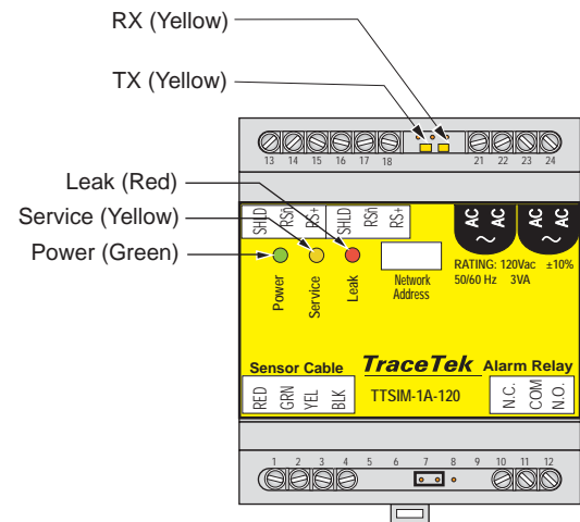
Figure 9. TTA-SIM-1A LED positions (all LEDs are located on the TTSIM unit)
