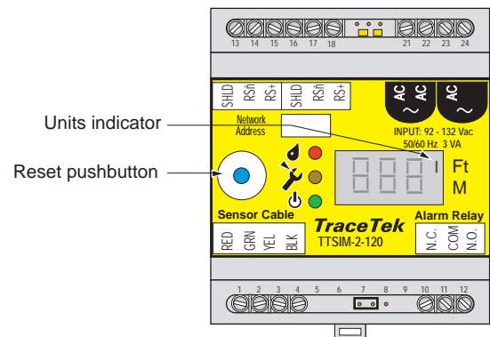
Figure 11. RESET pushbutton and units indicator locations
