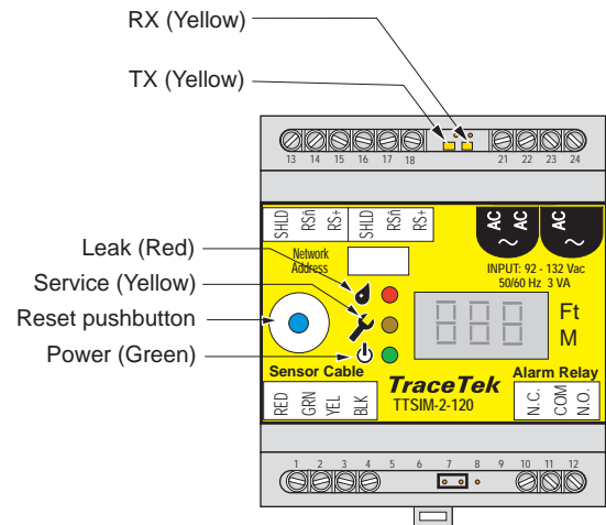
Figure 10. TTA-SIM-2 LED positions (all LEDs are located on the TTSIM unit)
