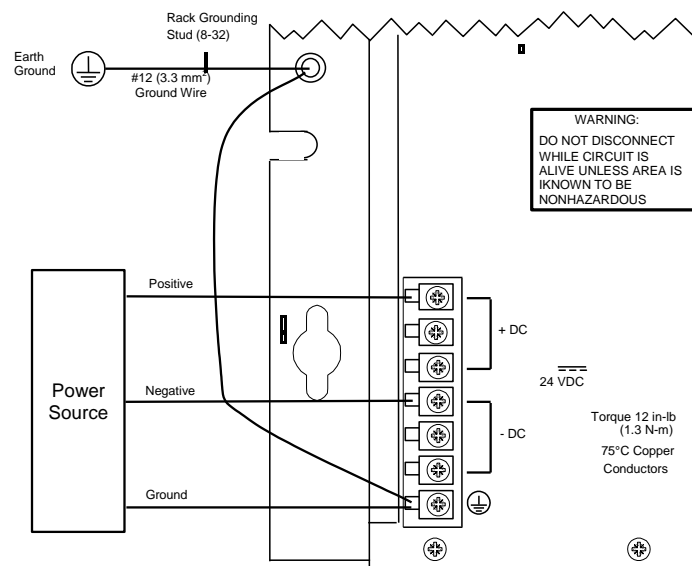
Terminal Board Connections for IC698PSD300
