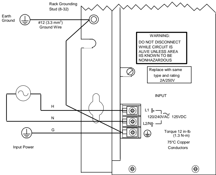
Terminal Board Connections for IC698PSA100/350
