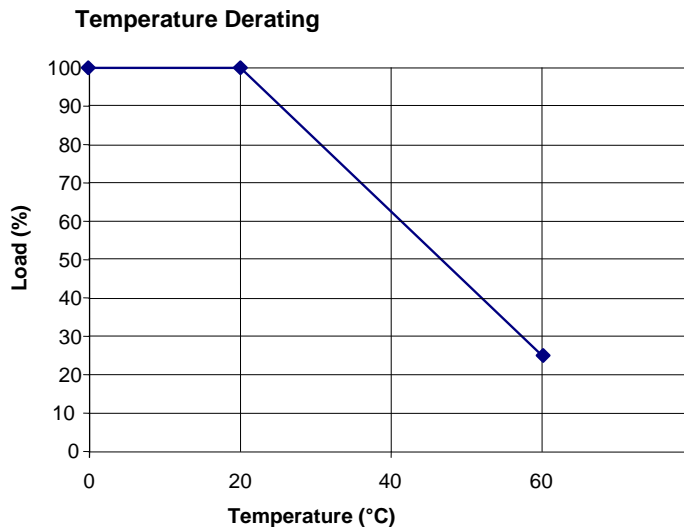
Temperature Derating Curve for IC698PSD300 without Forced Air Cooling
