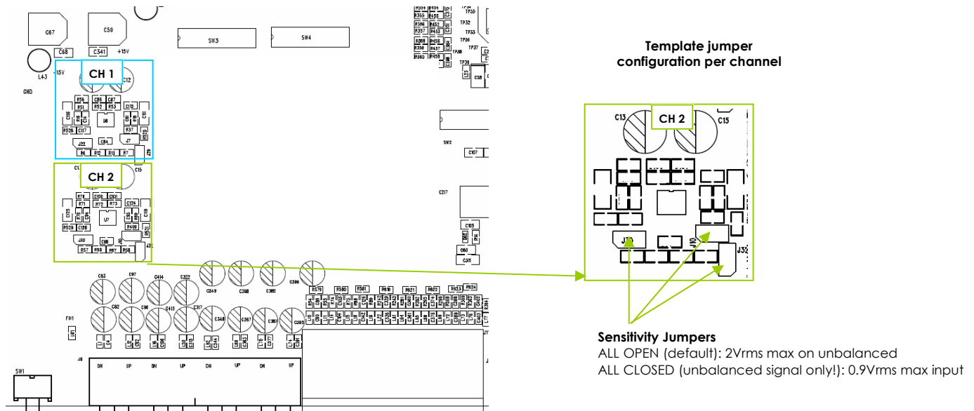
Board Layout arrangement for input jumper configuration
