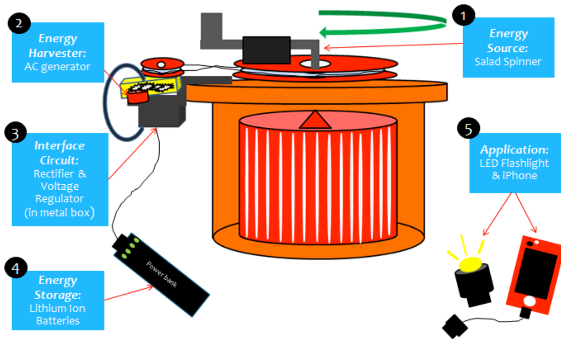
Figure 31 – Final UWash System Design
