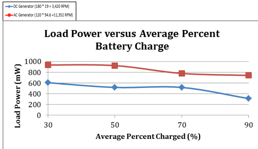
Figure 28 – Load power versus average percent battery charge
