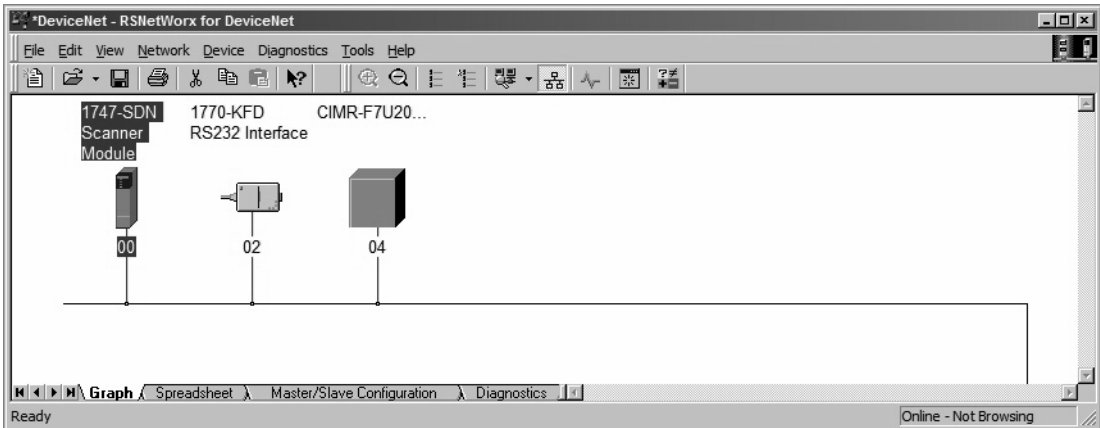
Fig 3.1 – Network Configuration
