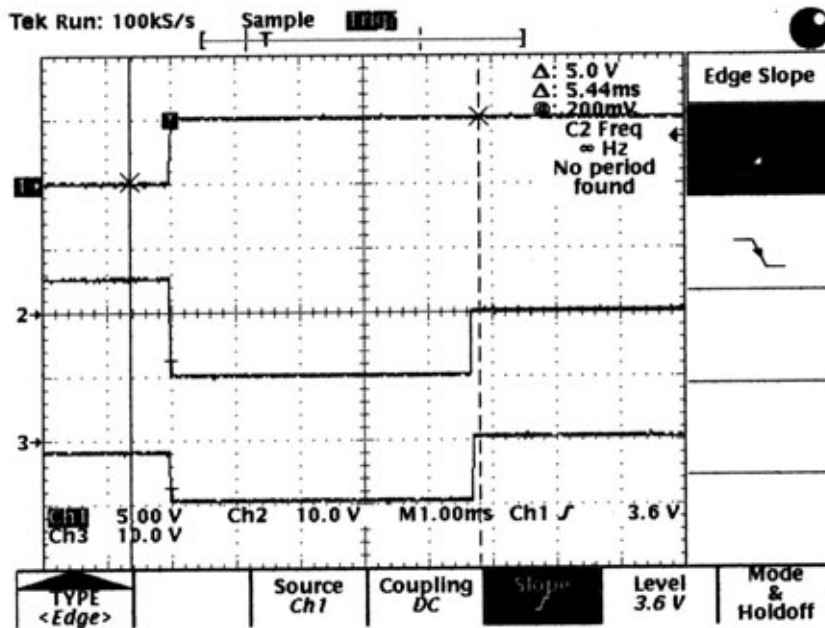
Figure 5.1—Normal reset sequence. Ch1 is the PC reset; Ch2 and Ch3 are arbitrary analog-output channels.
