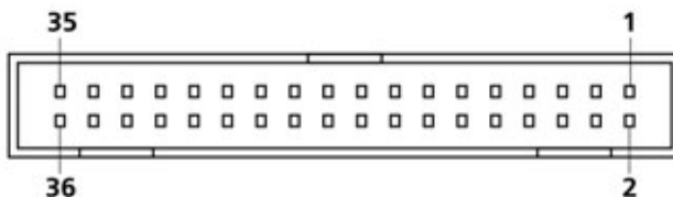
Figure 3.9—Physical layout of J2 on PD2-AO-8/16, -16/16 and -32 boards (view looking into the connector as mounted on the board).
