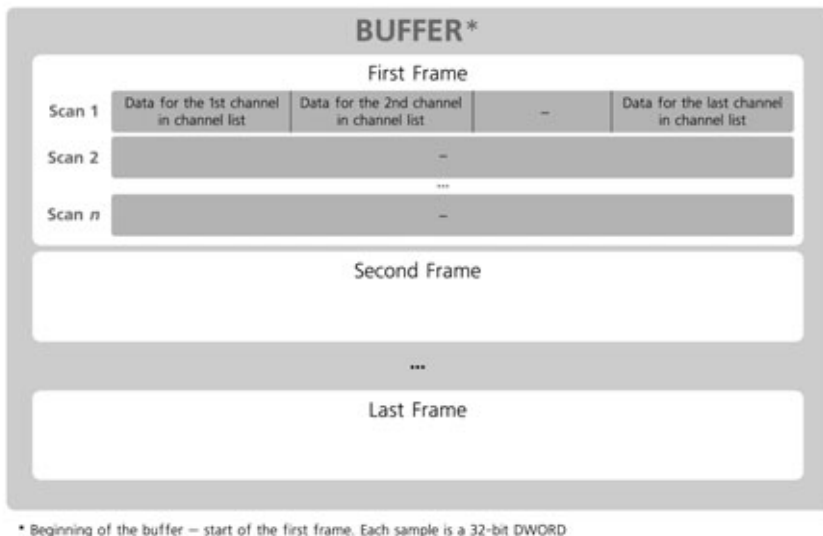
Figure 4.7—Graphical depiction of frames and scans.
