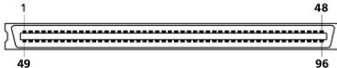
Figure 3.5—Physical layout of J1 on PD2-AO-8/16, -16/16 and -32/16 boards (view looking into the connector as mounted on the board).
