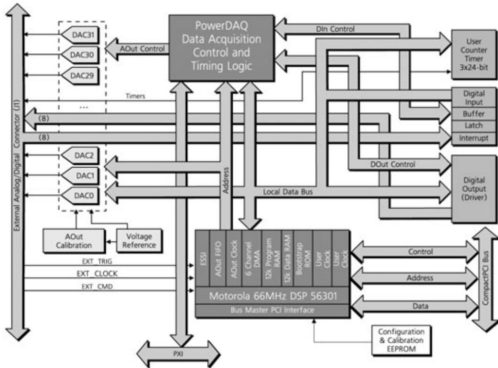
Figure 4.3—Block diagram of PowerDAQ PDXI-AO boards
