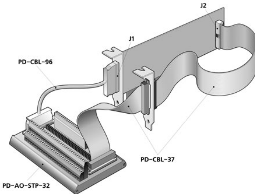
Figure 3.4—Connector layout for the PD2-AO-8/16, -16/16 and -32/16. J1 handles the analog outputs, while J2 carries digital I/O and interrupt signals.
