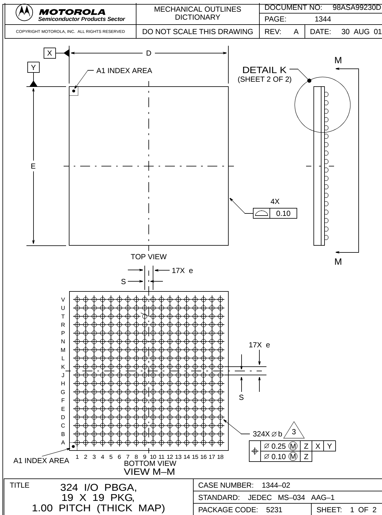
Figure 7-1. 324 MAPBGA Nomenclature
