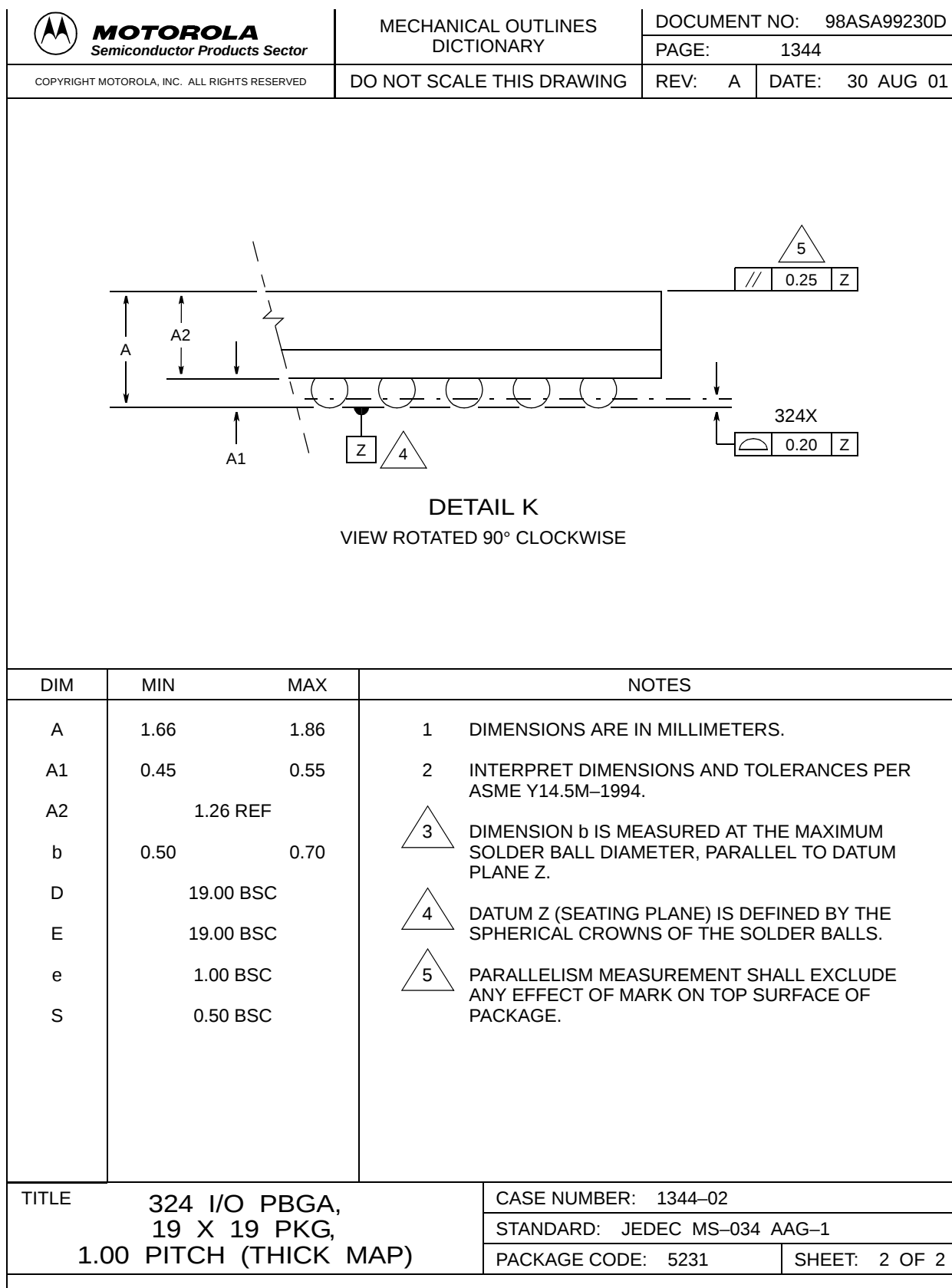
Figure 7-2. MAPBGA Dimensions
