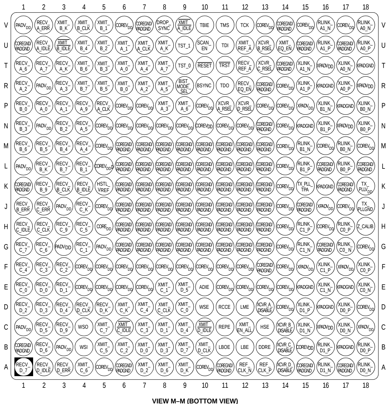
Figure 7-3. 324 MAPBGA Package
