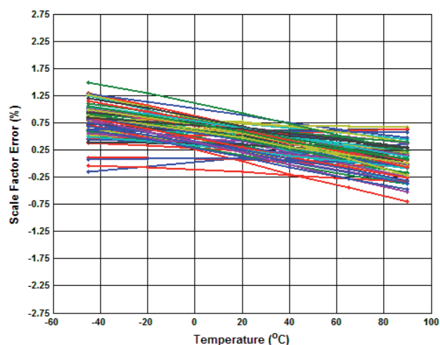
Figure 5.2 Gyroscope Scale Factor Error
