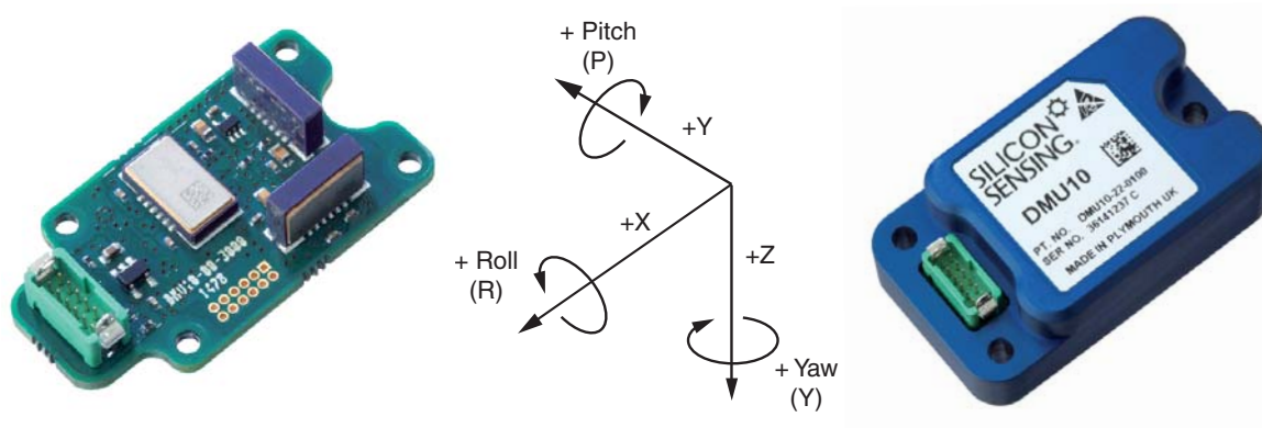
Figure 10.3 Axis Definitions
