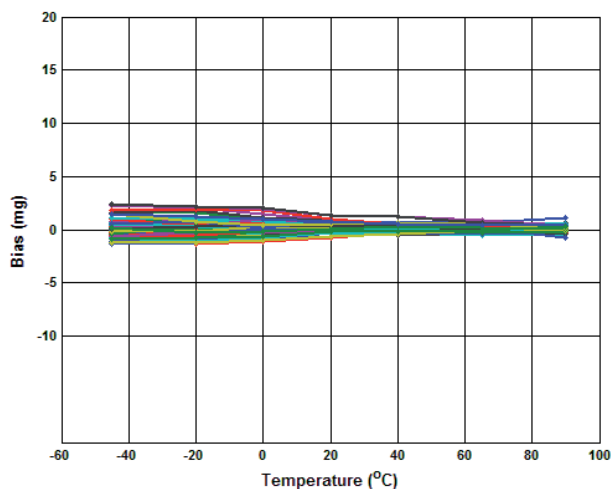
Figure 5.13 Accelerometer Bias
