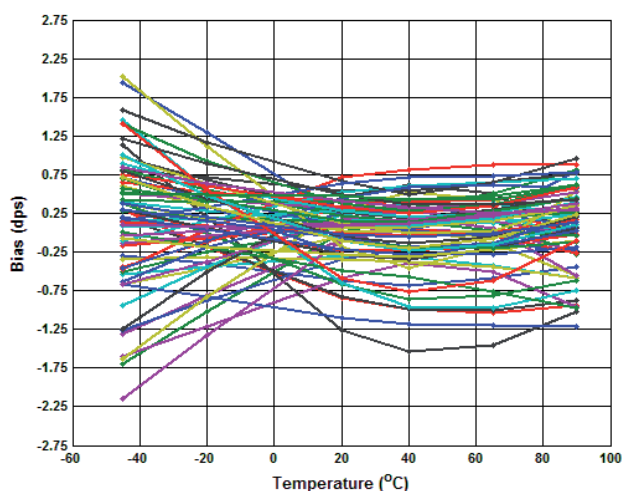
Figure 5.1 Gyroscope Bias
