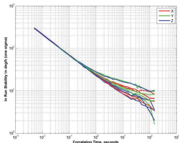
Figure 5.18 Gyroscope Stability
