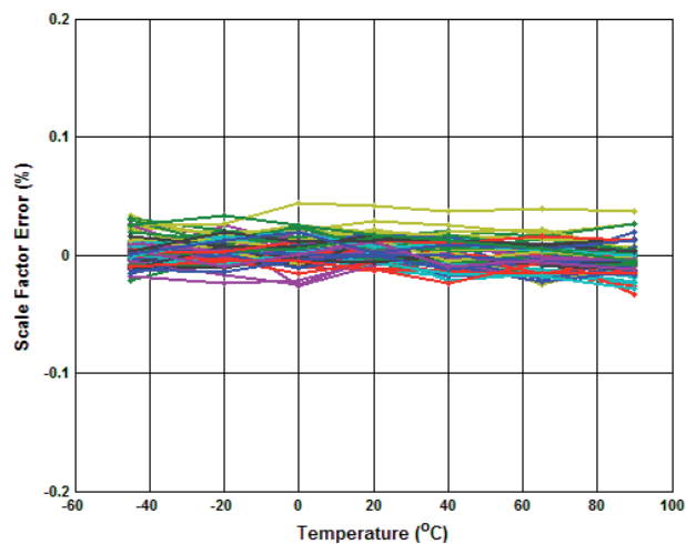
Figure 5.14 Accelerometer Scale Factor Error
