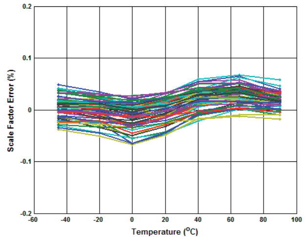
Figure 5.10 Gyroscope Scale Factor Error
