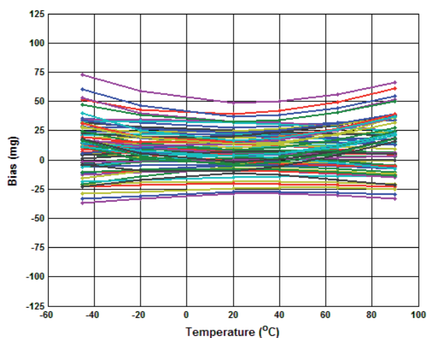
Figure 5.5 Accelerometer Bias
