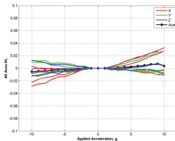
Figure 5.16 Accelerometer Non-Linearity Error
