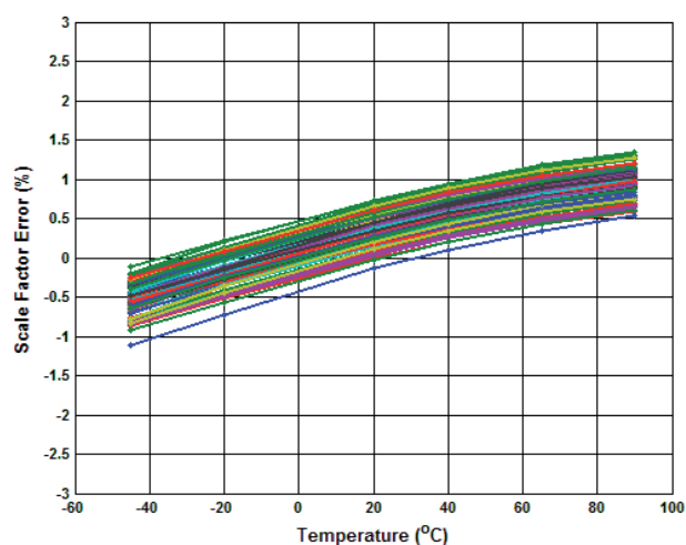
Figure 5.6 Accelerometer Scale Factor Error
