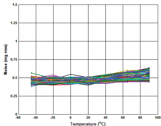
Figure 5.26 Accelerometer Noise over Temperature
