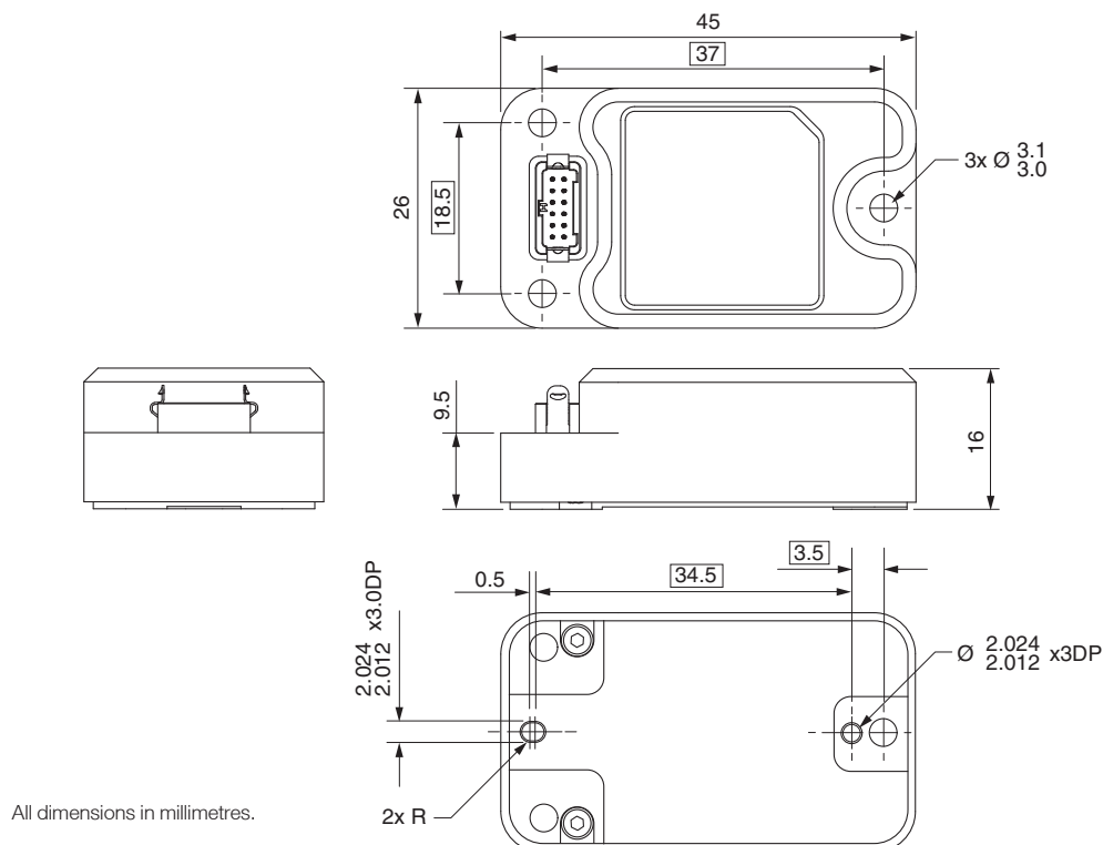
Figure 10.2 DMU10 (Module) Installation Drawing
