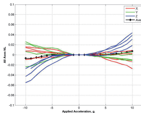
Figure 5.8 Accelerometer Non-Linearity Error
