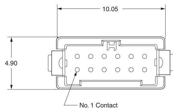
Figure 7.2 Male Connector DMU10
