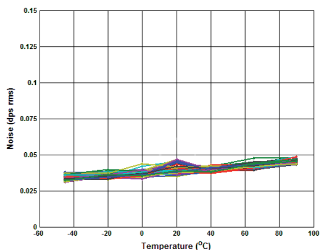
Figure 5.21 Gyroscope Noise over Temperature
