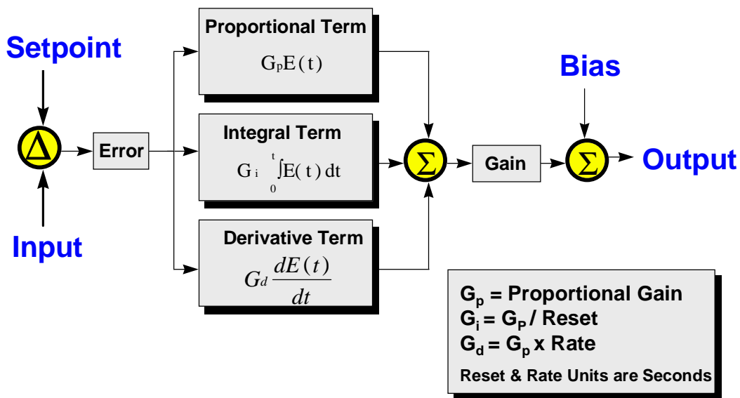
Figure 9- 1. PID Algorithm
