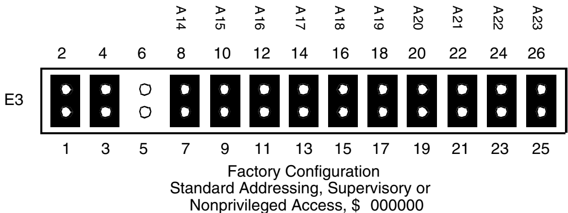
Figure 2-4: Board Configuration Jumpers
