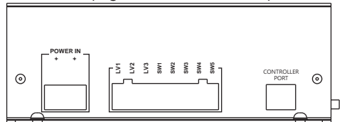
front view (Light control connector)
