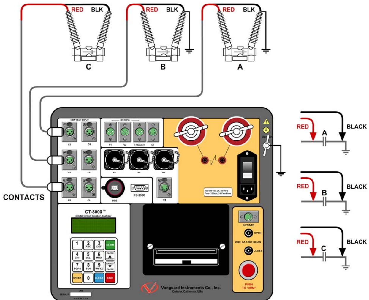
Figure 3. Typical 3-Phase Circuit Breaker Connections
