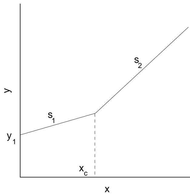
Figure 13.2 Parameters of the two line model.
