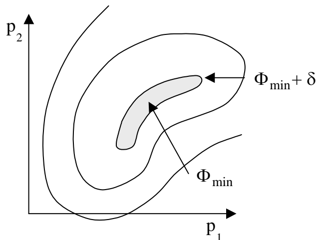
Figure 6.1. Objective function contours in parameter space; linear model.
