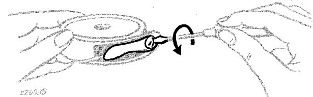
Fig. 28. Decreasing Bobbin Thread Tension
