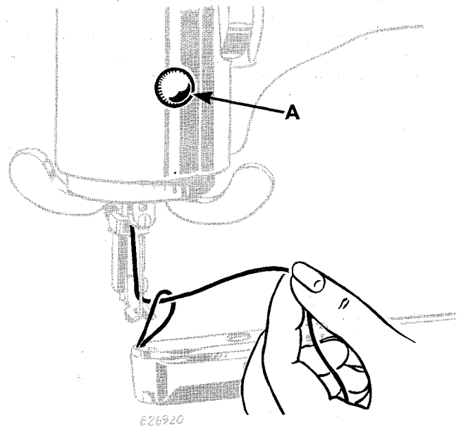
Fig. 22. Drawing up Bobbin Thread
