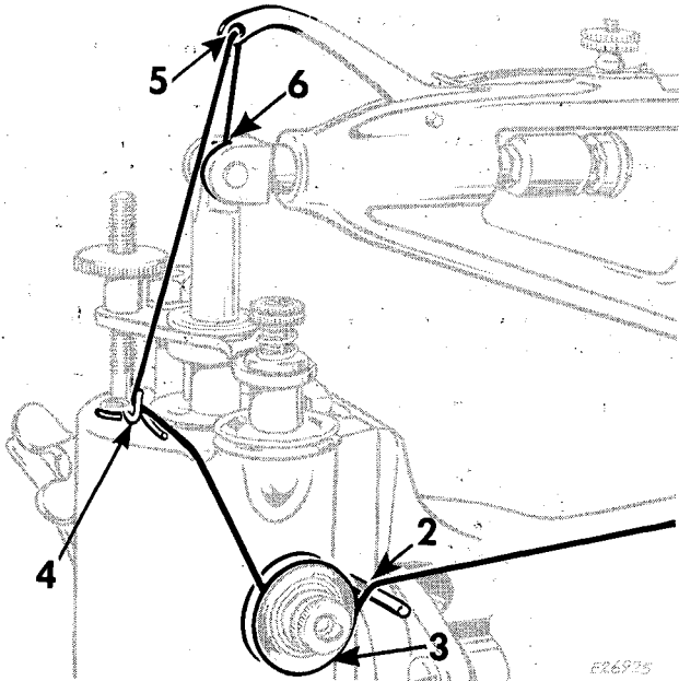
Fig. 21. Upper Threading for Darning
