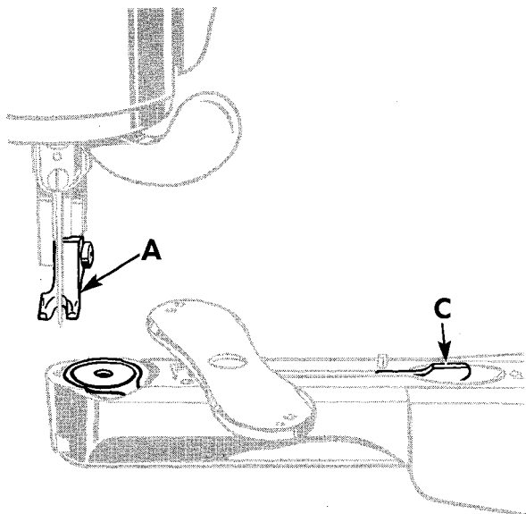
Fig. 17. Replacing Shuttle
