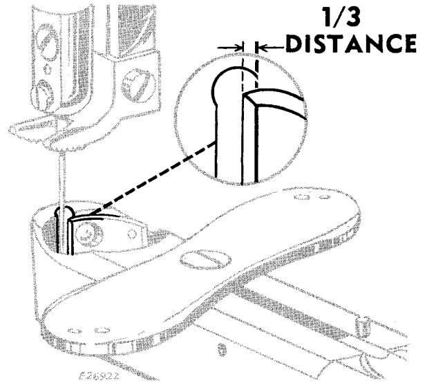
Fig. 38. Correct Timing of Shuttle Carrier
