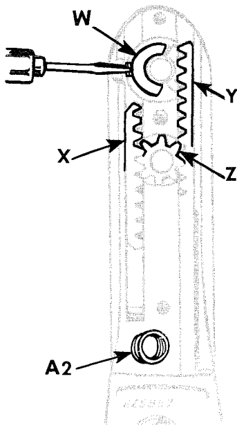
Fig. 35. Removing Parts from Rack Box
