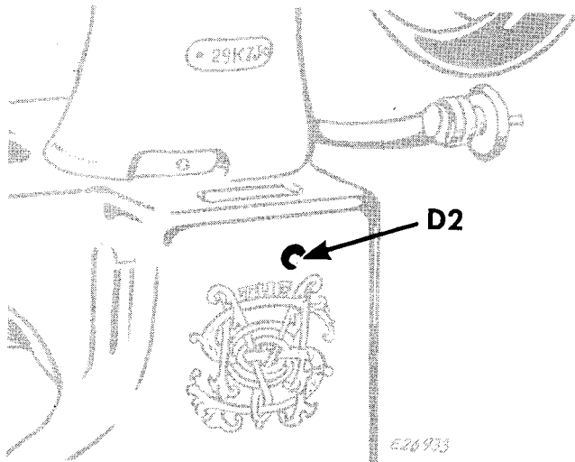
Fig. 37. Location of Eccentric Stud for Timing Shuttle
