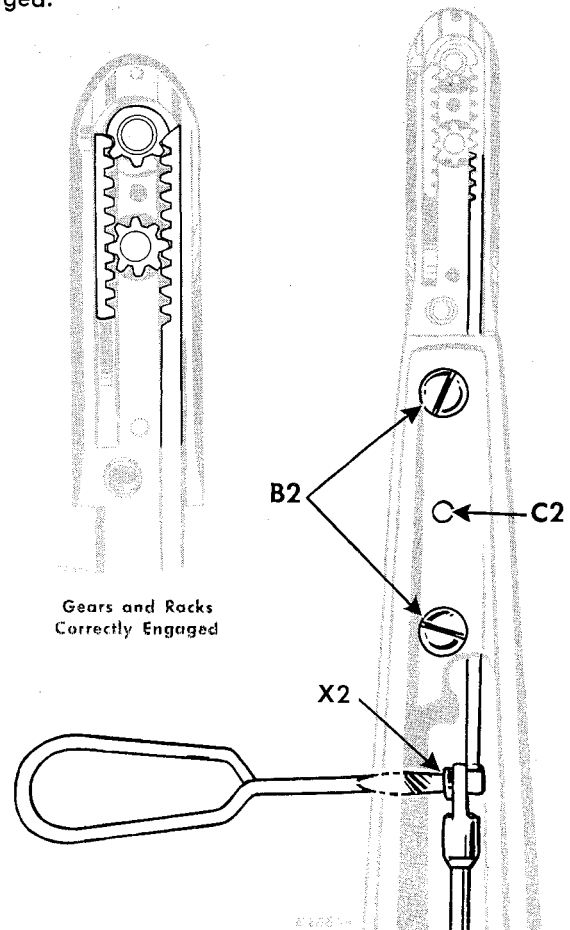
Fig. 36. Removing Rack Box
