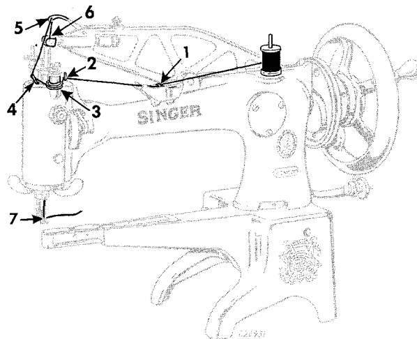
Fig. 19. Threading Needle
