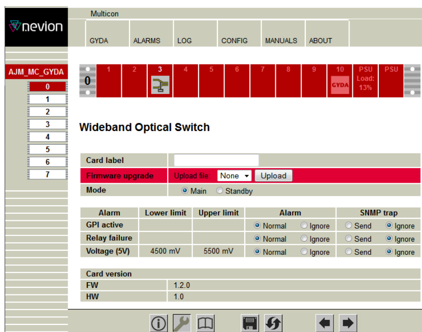
Figure 19: Config page
