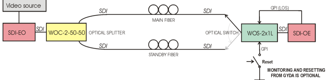
Figure 3: Possible setup for APS functionality, standby fiber is not monitored.
