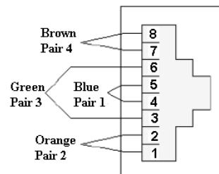
Figure 10: GPI Outlet
