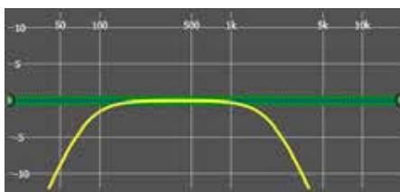
Crossover Frequency 80 - 2000 Hz @ 12 dB Oct.
