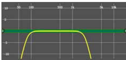
Crossover Frequency 80 - 2000 Hz @ 24 dB Oct.
