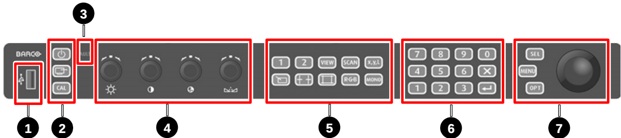
Figure 27: Control panel
