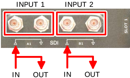
Figure 9: Input connectors SDI input board
