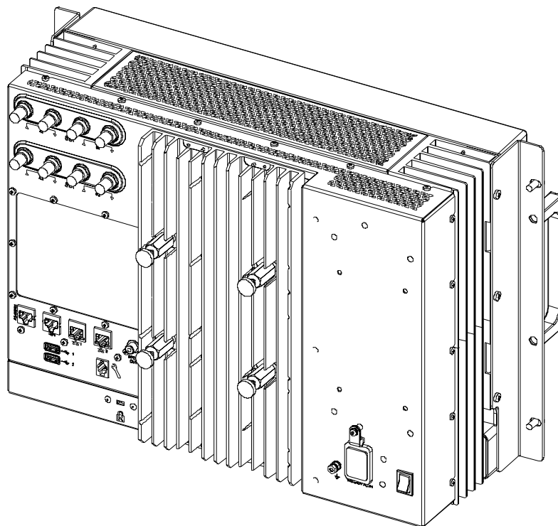
Figure 68: RHDM-1701 3D rear view
