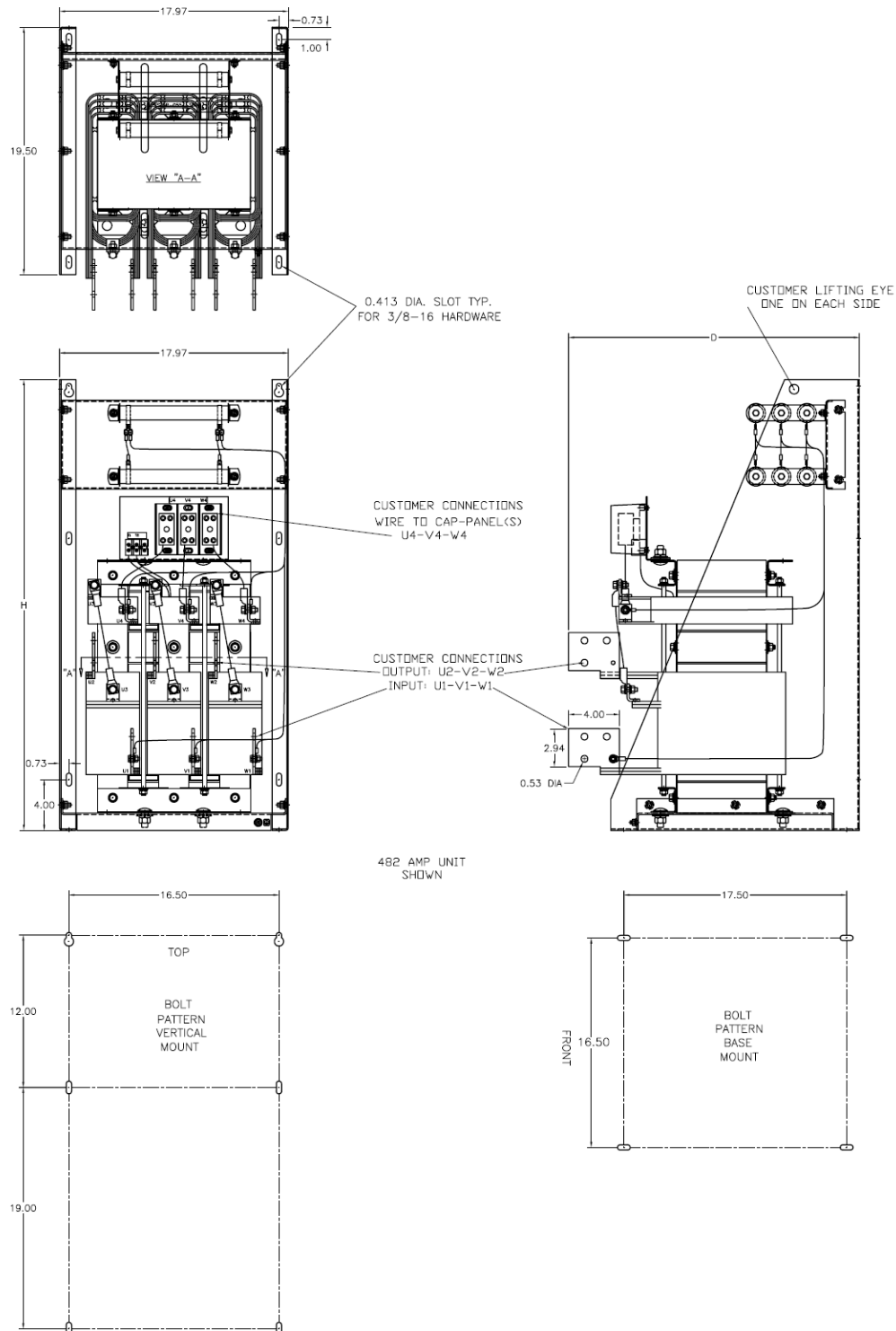
Figure 8 320 – 482 AMP
