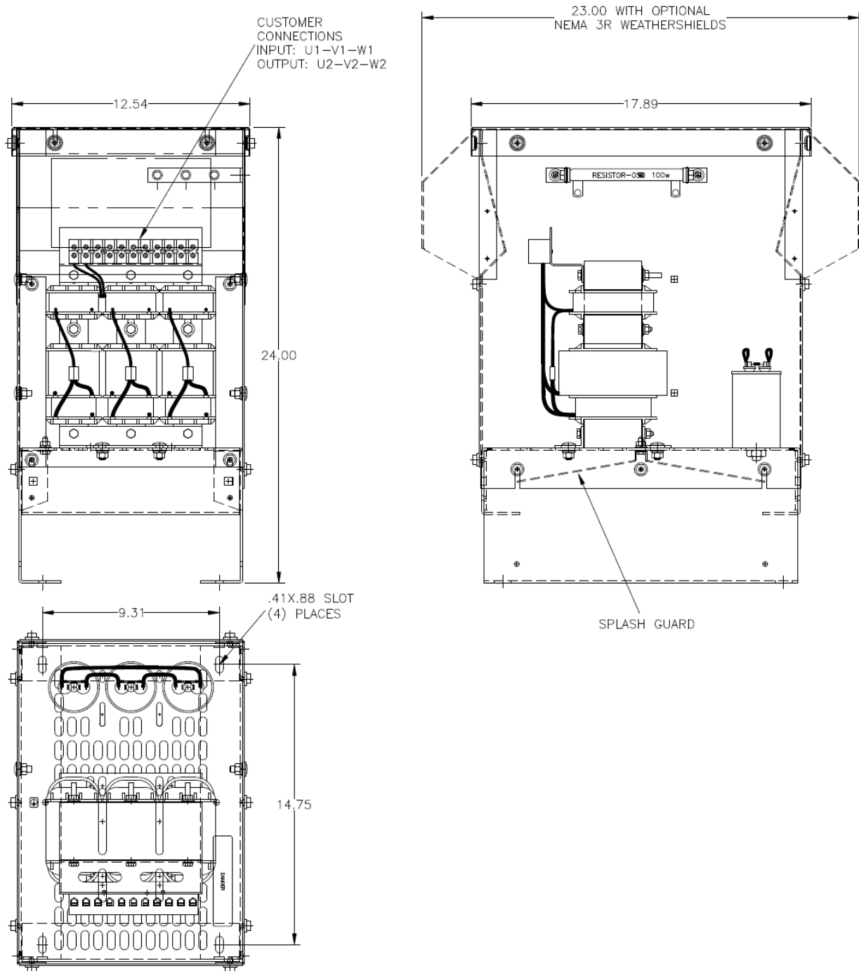
Figure 17 6 - 44 AMP
