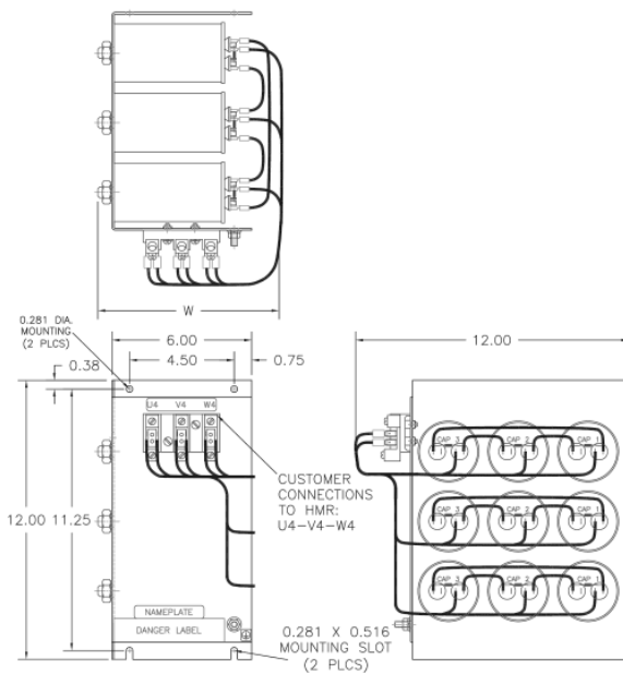
Figure 14 9 Caps
