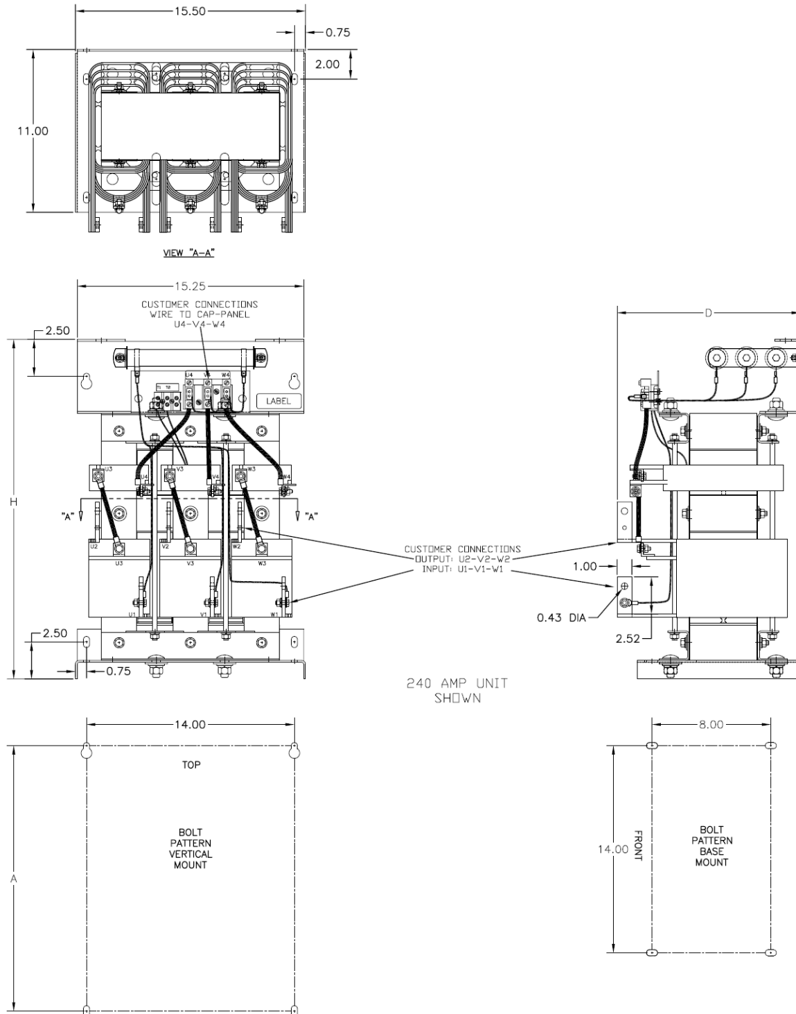
Figure 7 128 – 240 AMP
