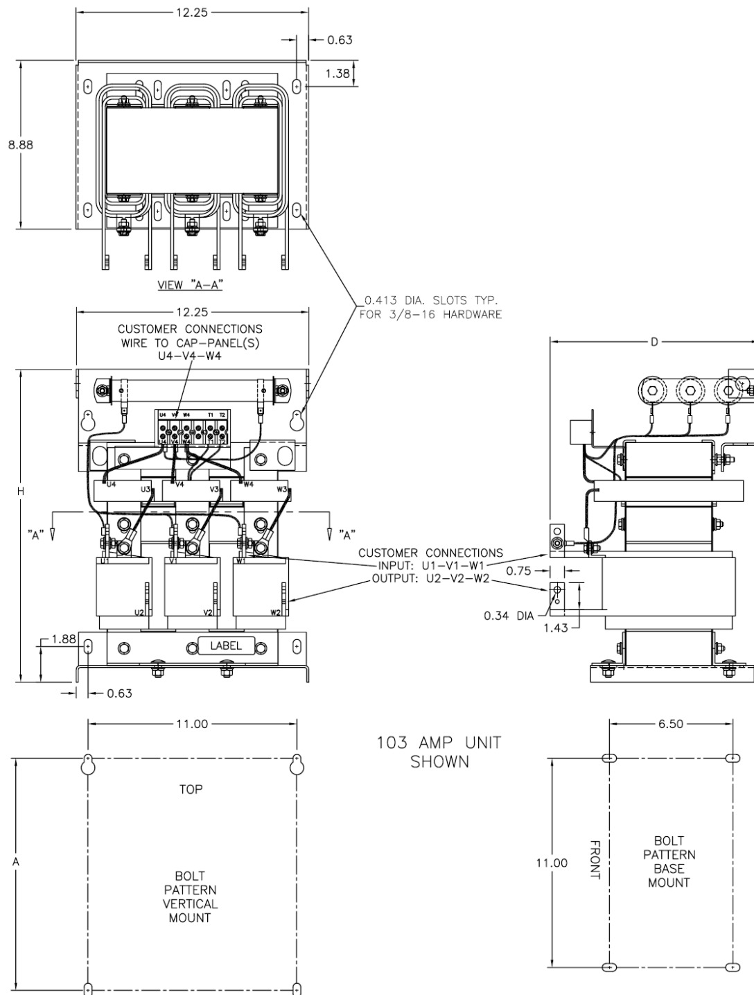
Figure 6 52 – 103 AMP
