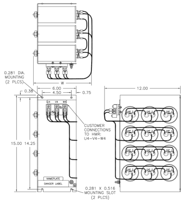
Figure 15 12 Caps
