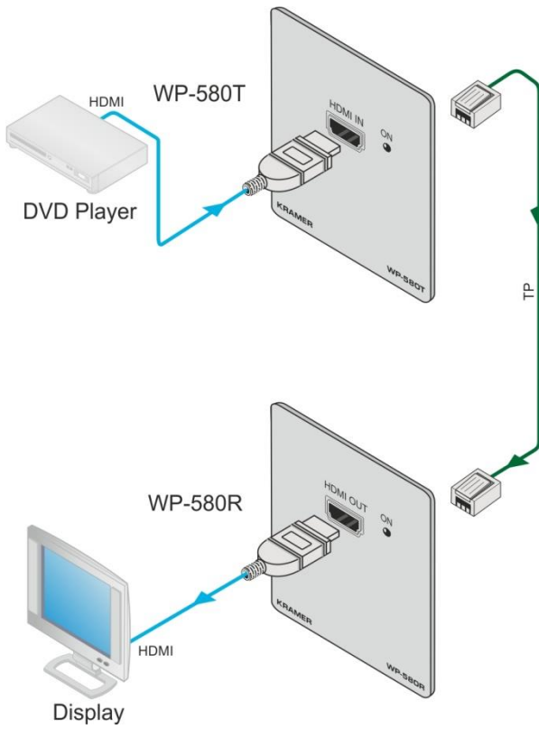
Figure 5: Connecting the WP-580T/WP-580R Transmitter/Receiver
