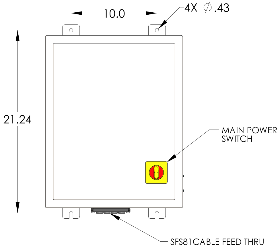
Figure 4. Electrical Control Box Mounting
