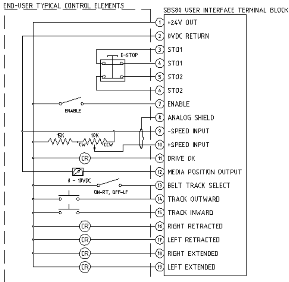
Figure 2. SBS81 Typical User Interface Schematic
