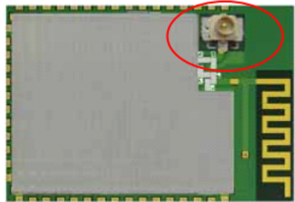
External:I-PEX
