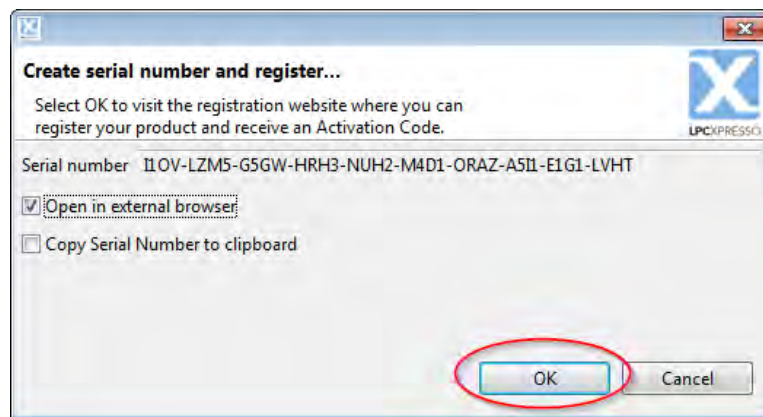
Fig 18. Product activation
