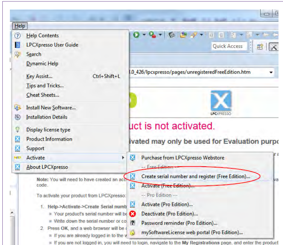
Fig 17. Product activation
