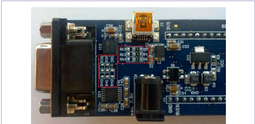
Fig 11. Solder jumpers for additional interface configuration
