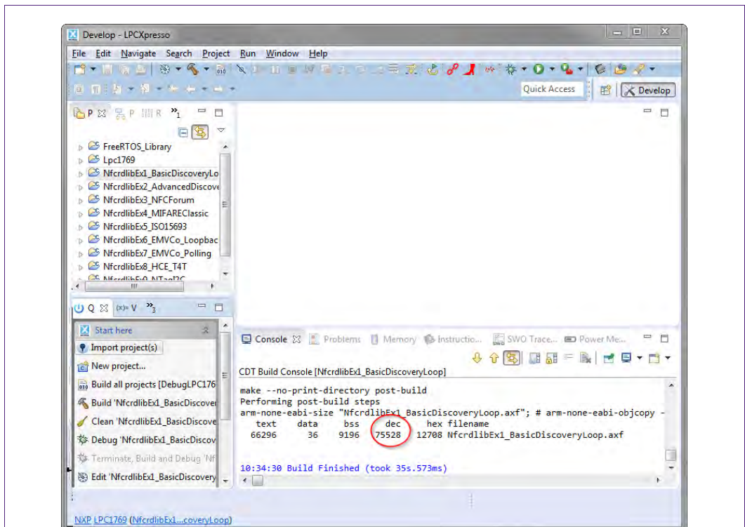
Fig 24. After the build process one can see the size of the image in the console window.
