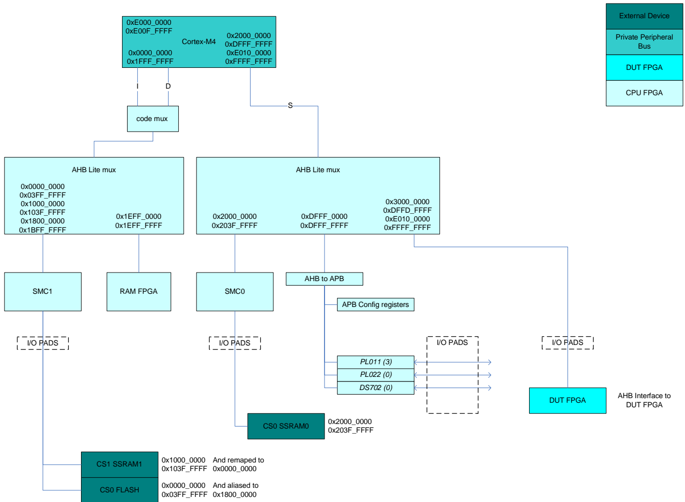
Figure 4: CPU FPGA Bus Architecture
