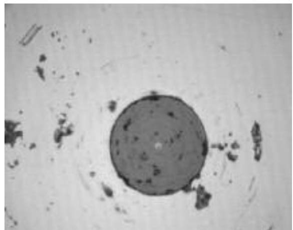
Contaminated Connector End-Face | Photo NS134
