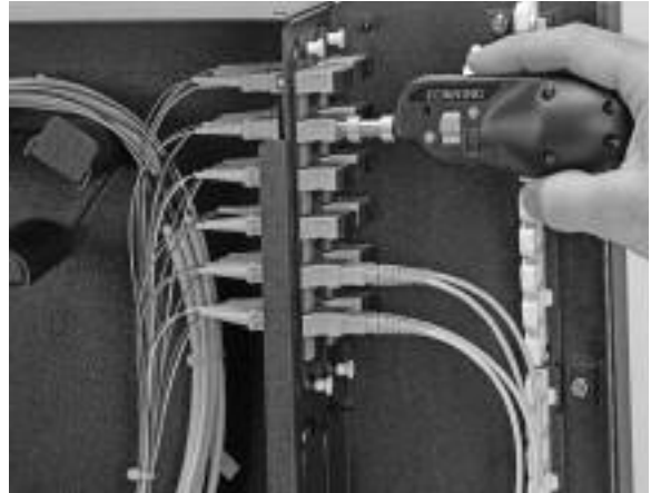
Video Probe in Patch Panel | Photo TEQ36
