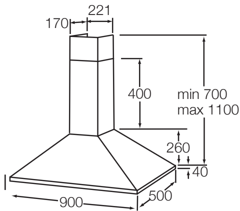
STANDARD CANOPY
