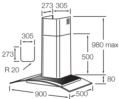
GLASS CANOPY
