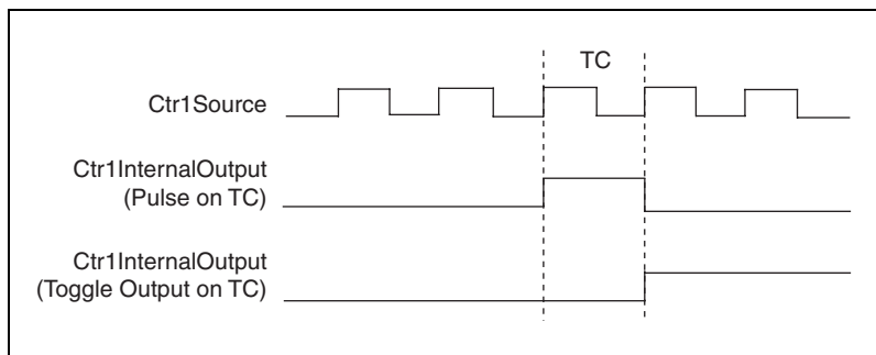
Figure 5-9. Ctr1InternalOutput Behavior
