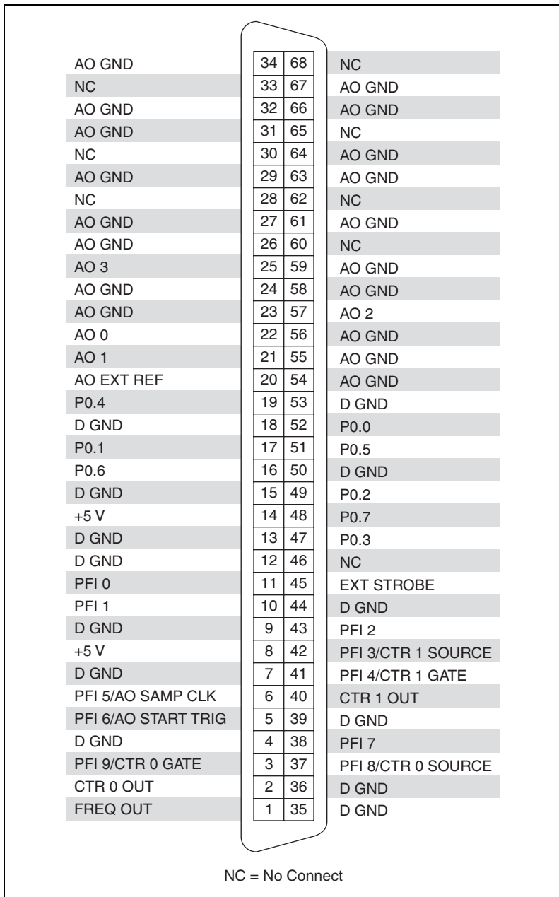
Figure 2-1. NI 6711/6731 68-Pin AO I/O Connector Pinout
