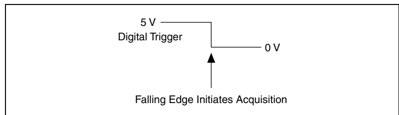
Figure 10-1. Falling-Edge Trigger
