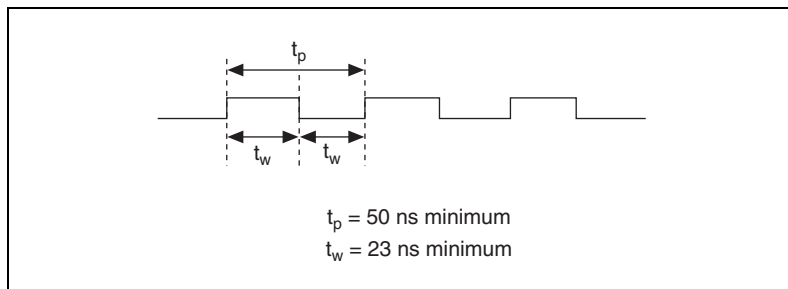
Figure 5-10. MasterTimebase Timing Requirements
