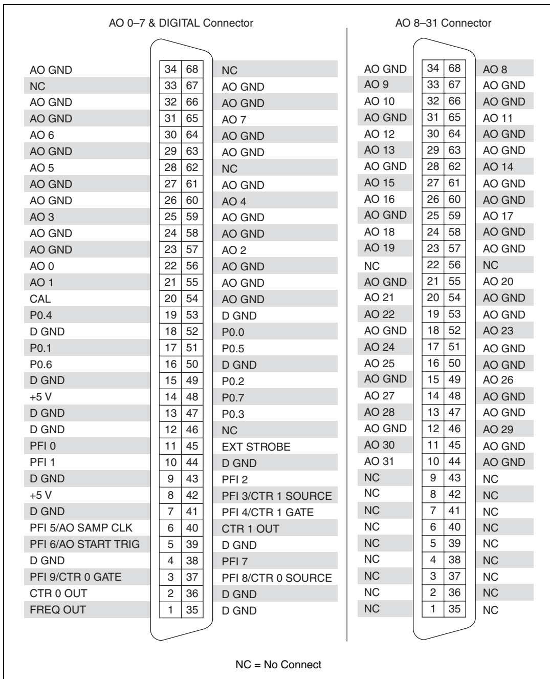
Figure 2-4. NI 6723 68-68-Pin Extended AO I/O Connector Pinout
