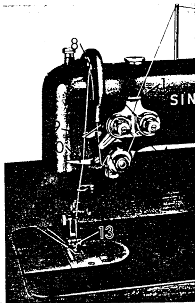
Fig. 7 Upper threading
