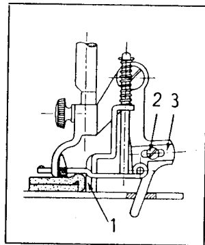
← Fig. 72 Setting the felling foot pressure plate
