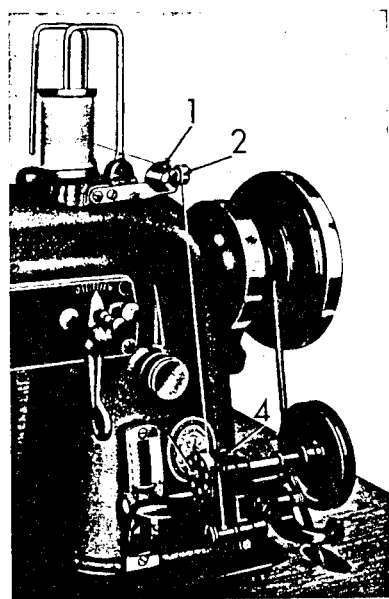
Fig. 8 Bobbin winding, treadle operated --
