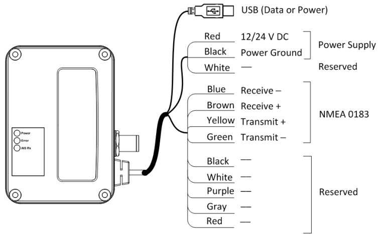
Figure 7 Wiring Instructions
