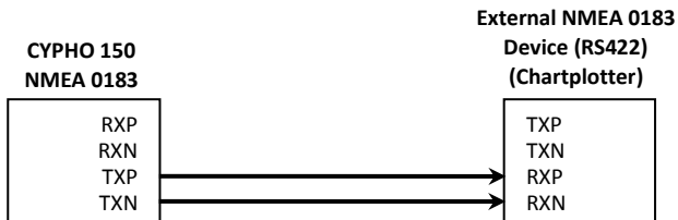
Figure 8 NMEA 0183 Connection illustration
