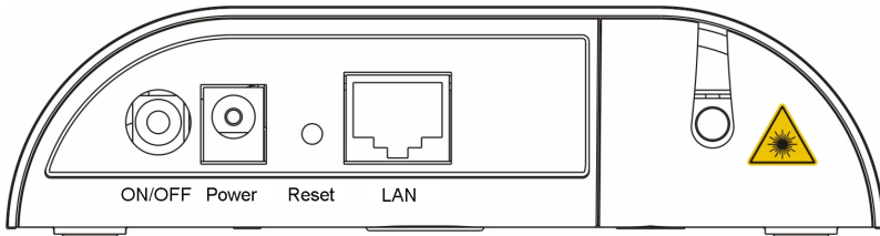
Figure 2-2 Front view of the AN5506-01-A rear panel
