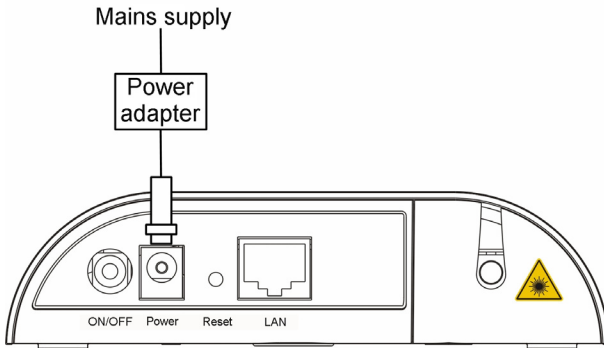
Figure 3-3 Connection diagram for power cables
