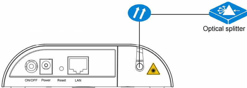
Figure 3-1 Connection diagram for optical fiber
