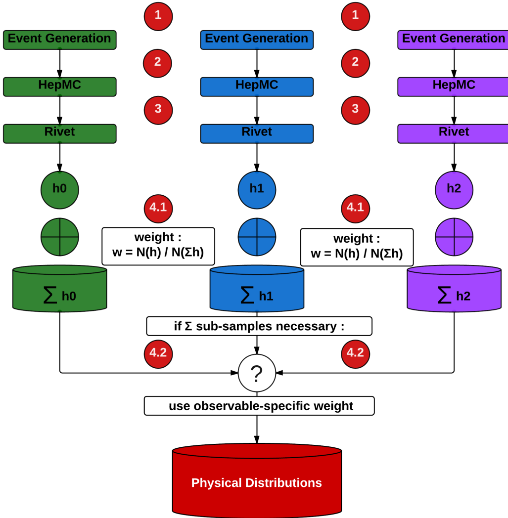
Figure 11: A schematic representation of the path from the Event Generation to the Physical Distributions produced within the MCPLLOTS framework. The sequential steps are labelled 1 – 4. Their technical implementation in the MCPLLOTS framework is described in section 6.
