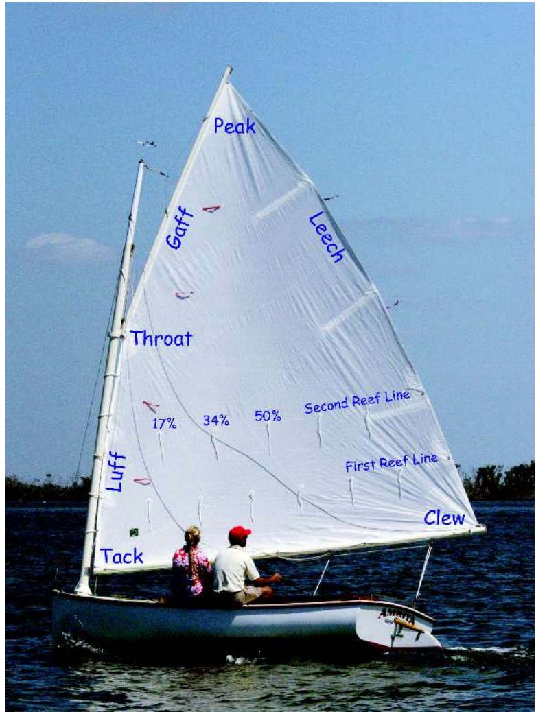
A look at the parts of a four-sided gaff-rig sail reveal similarities to the more familiar three-sided sail, with a few additional points. The reef points divide the sail lengthwise, and can be used to measure the position of the draft.
