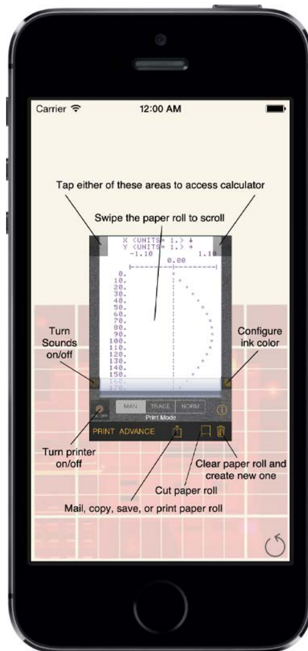
Printer Information View
