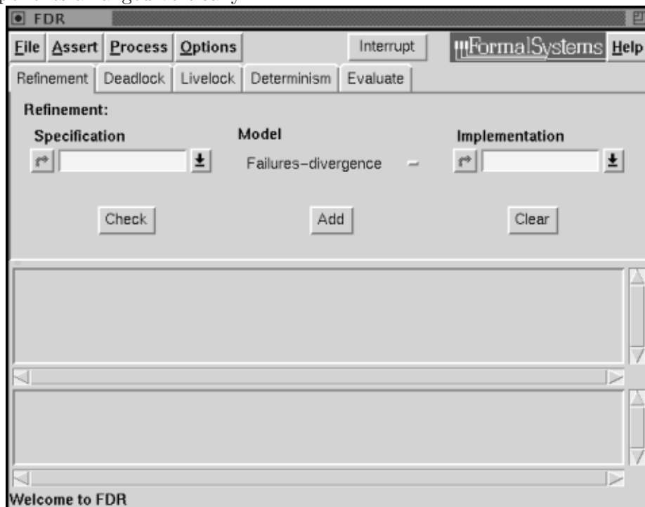
Figure 3: Main Window
