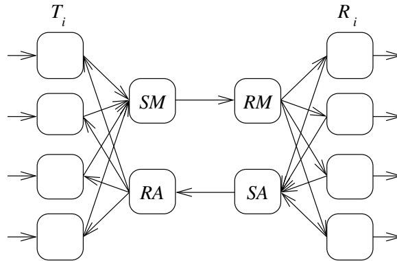
Figure 2: Multiplexed Buffers with Acknowledgement
