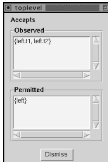
Figure 7: Acceptances Comparison Window
