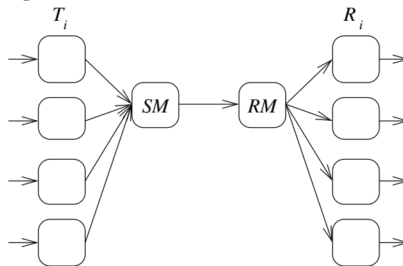
Figure 1: Multiplexed Buffers
