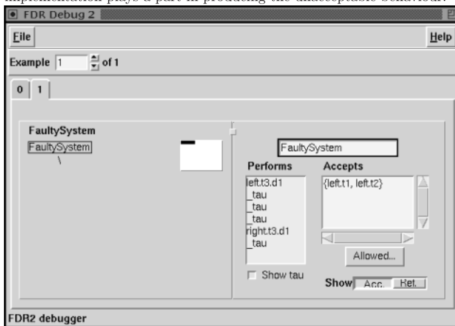
Figure 6: Debugging Window
