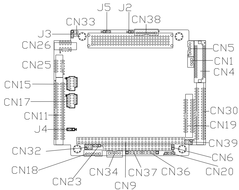
Figure 2.1 Connectors (component side)
