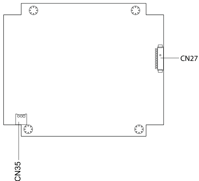
Figure 2.2 Connectors (solder side)
