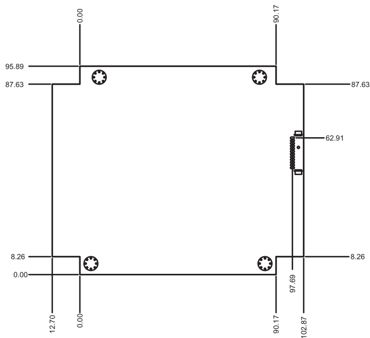
Figure C.1 PCM-4153 Mech drawing (comp side)
