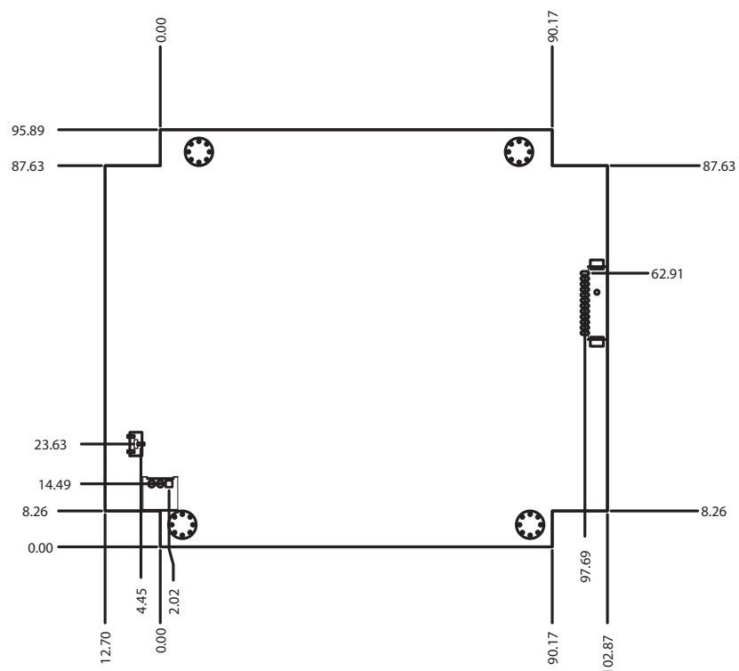
Figure 1.2 Board layout: dimensions (solder side)
