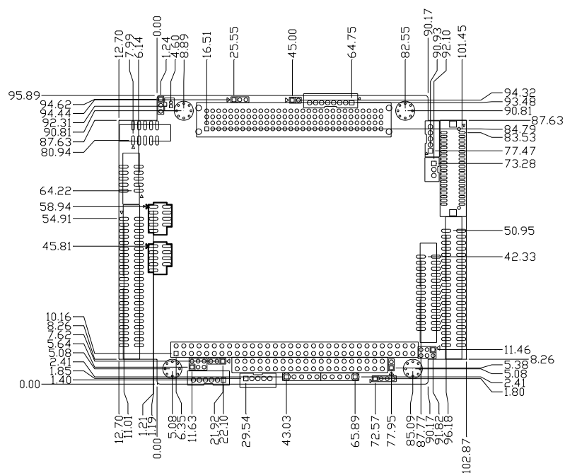
Figure C.1 PCM-4153 Mech drawing (comp side)
