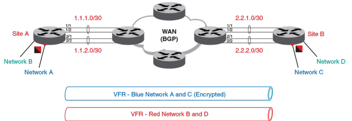
FIGURE 5 IPsec network diagram
