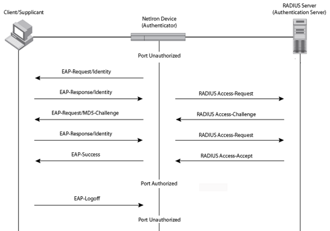
FIGURE 11 Message exchange during authentication
