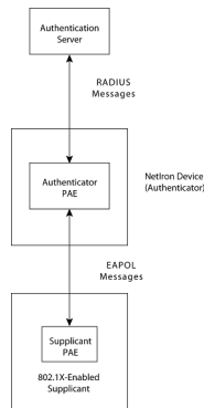
FIGURE 9 Authenticator PAE and supplicant PAE
