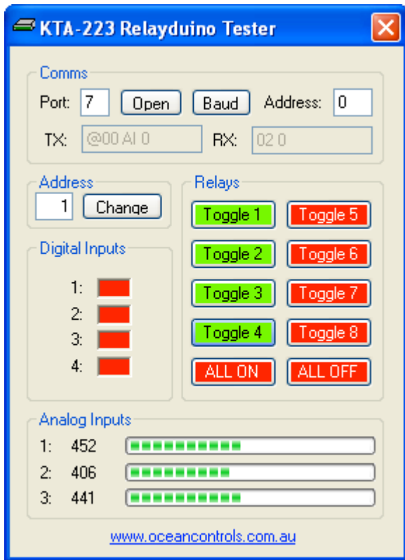
Figure 2 - Windows Test Utility
