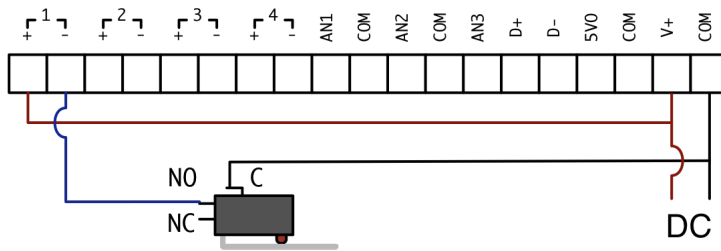
Figure 3 - Wiring a dry contact switch
