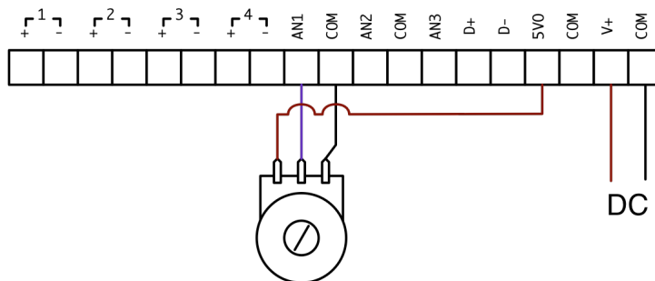
Figure 6 - Wiring a potentiometer
