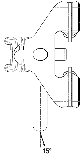
Harken HC9606 cars beginning with A0633 and B0768 with 8 mm shackles have the ability to handle loading at an angle up to 15° beyond vertical. Loads beyond 15 degrees from vertical will overload car.
