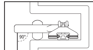
Mounted in recess: cars with wheel toggle for loading over an edge
