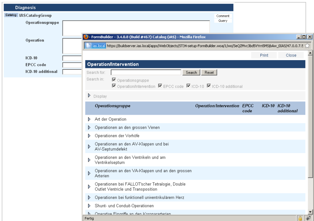
Fig. 22: Example of the view of an IASCatalogGroup with catalog pop-up (excerpt).
