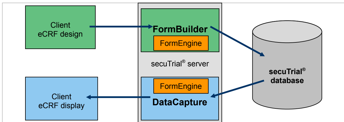
Fig. 1: Schematic depiction of eCRF generation. In the FormBuilder, the FormEngine is also used to preview the eCRF.
