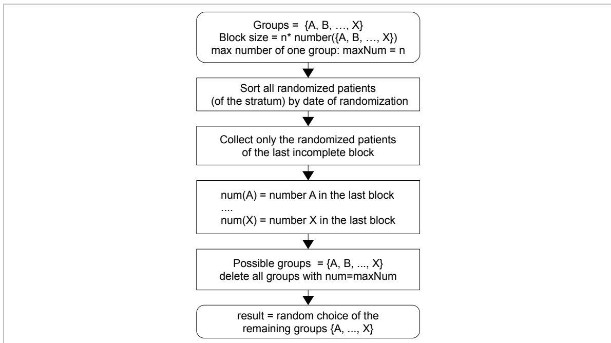
Fig.44: Determination of randomization with “Extended Stratified Block without list (secuTrial)” algorithm.
