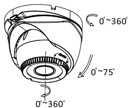
Figure 2-3 3-axis Adjustment
