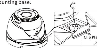
Figure 2-2 Release The Lock Screw
