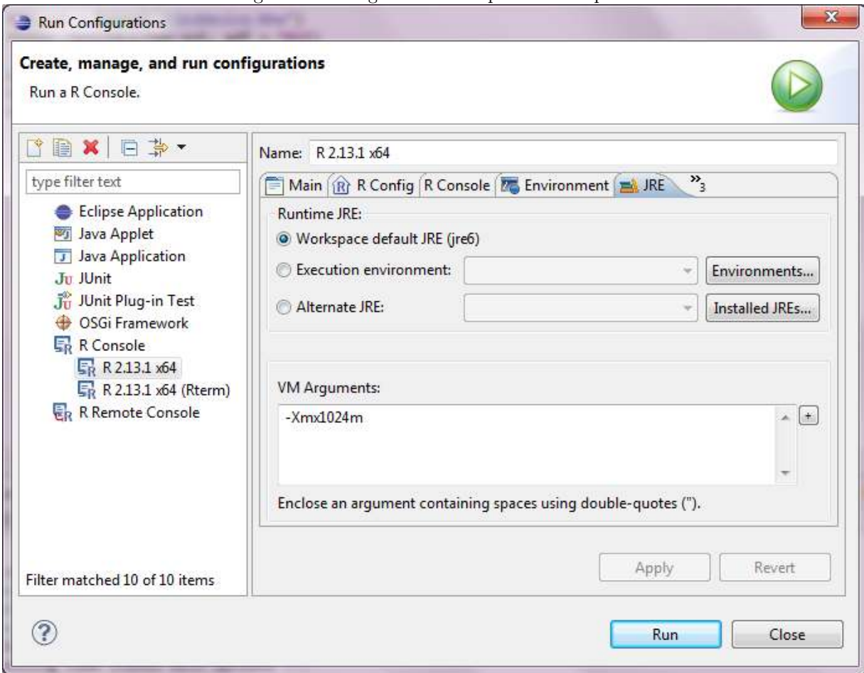
Figure 3: Setting the Java heap size in Eclipse:
