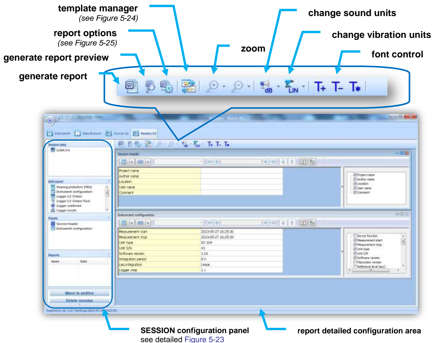
Figure 5-22 SUPERVISOR main SESSION window
