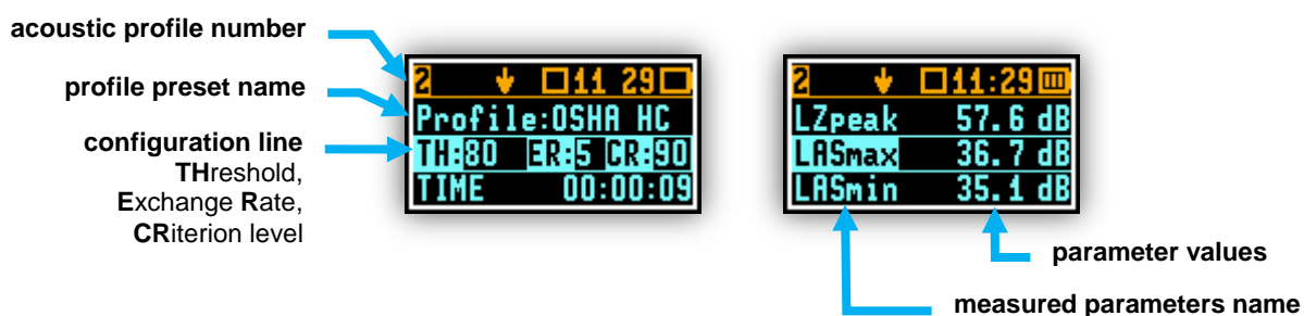
Figure 3-12 Results list view mode screens
