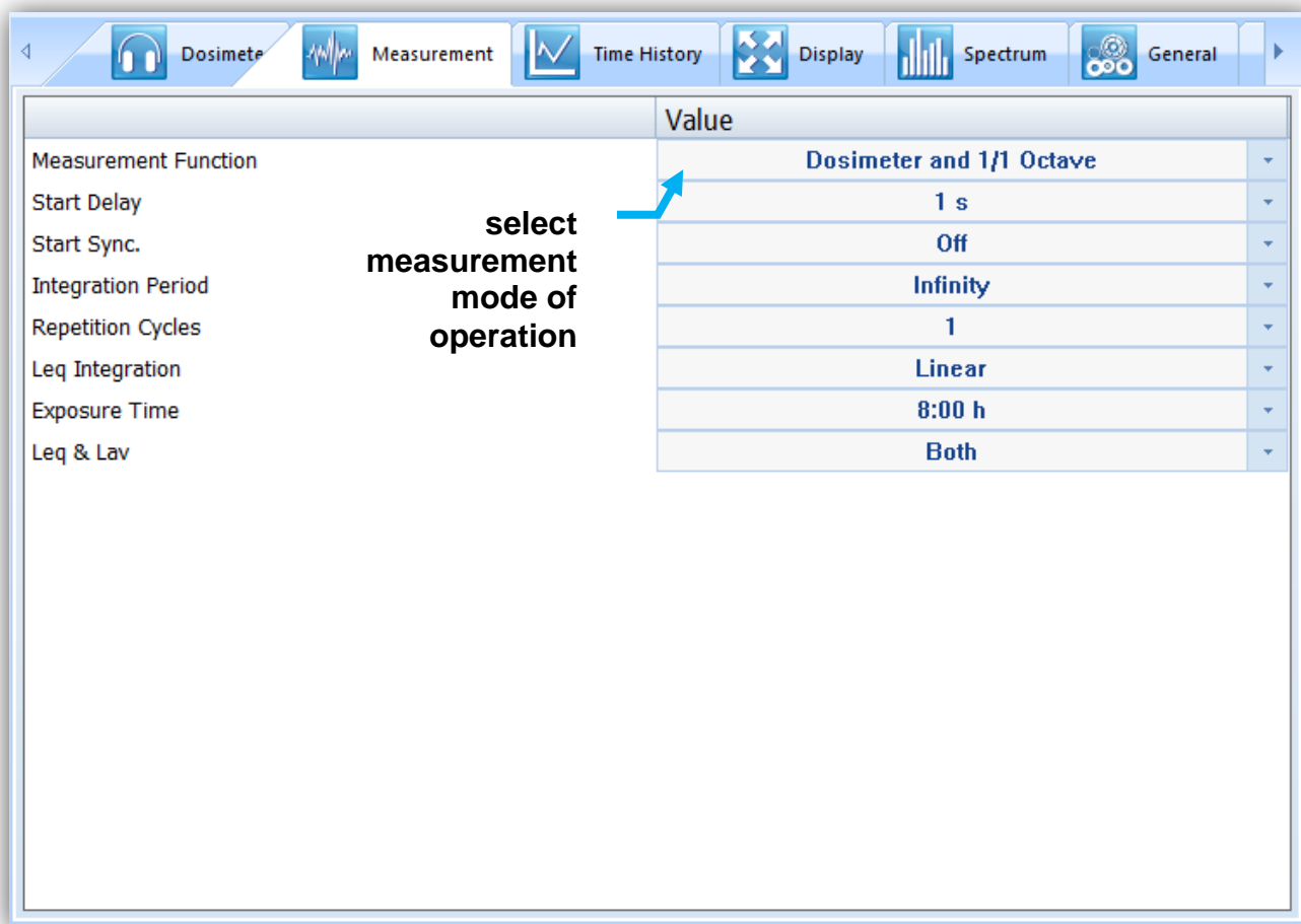
Figure 5-8 Measurement configuration settings tab
