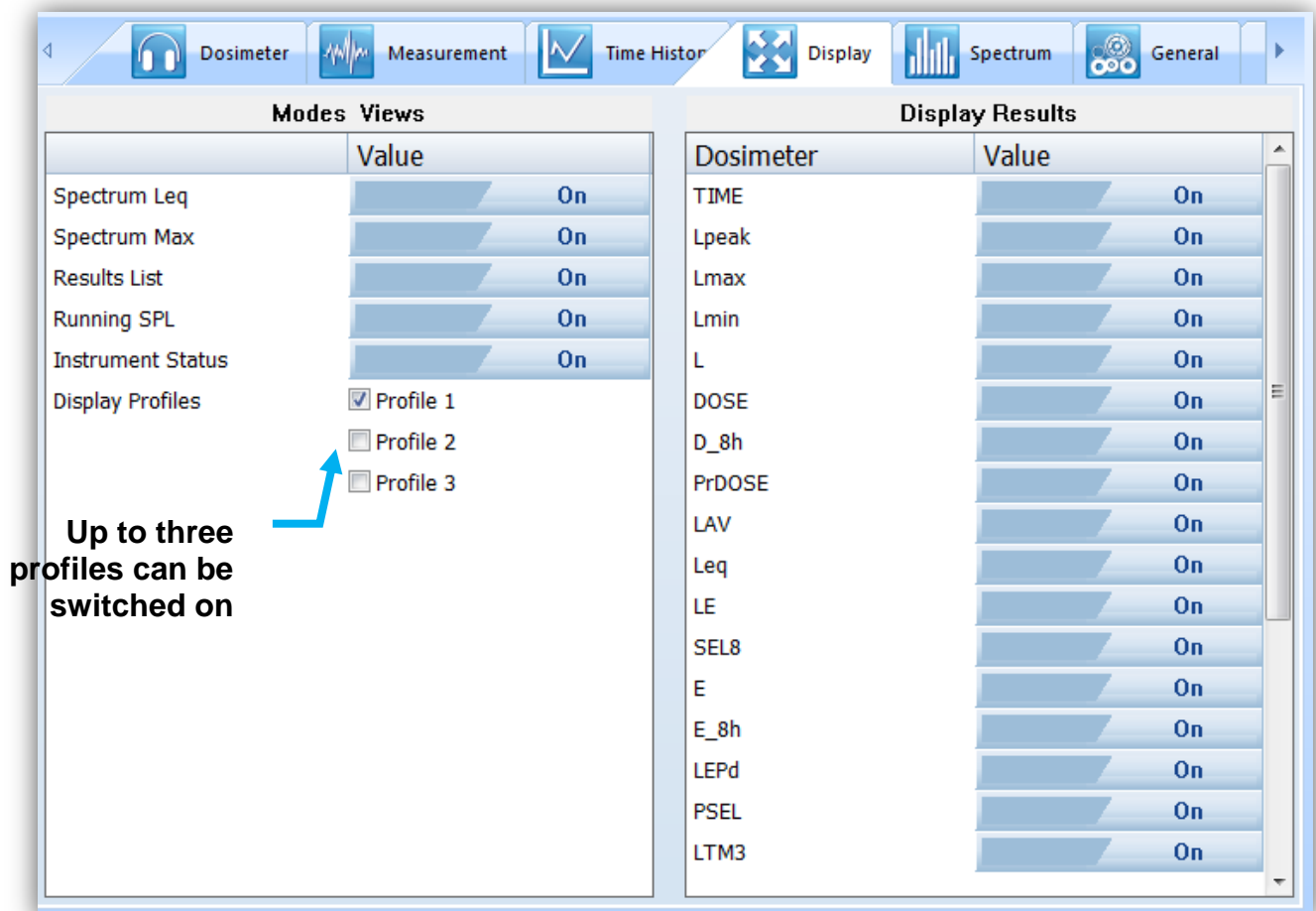
Figure 5-10 Display VIEW configuration tab
