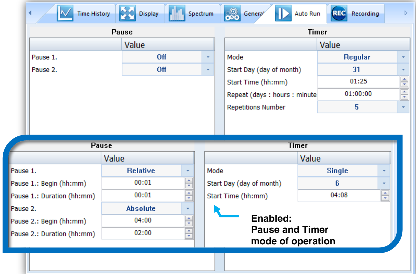
Figure 5-17 Auto-run configuration tab
