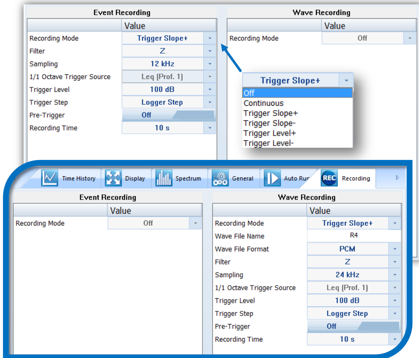
Figure 5-18 Audio Event and Wave recording configuration panels
