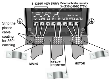
Figure 11: Vacon 20 power connections, MI2 - MI3
