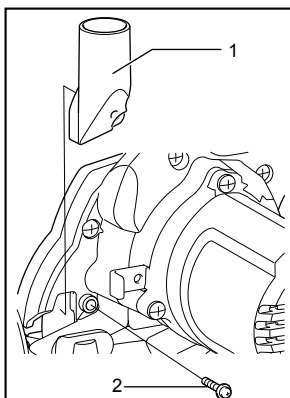
1. Dust nozzle (accessory) 2. Screw
