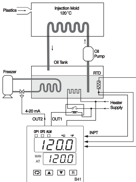
Figure 4.3 Heat-Cool Control Example
