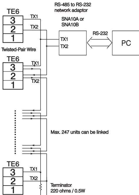
Figure 2.21 RS-485 Wiring
