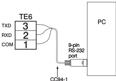
Figure 2.22 RS-232 Wiring
