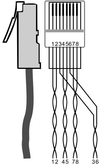
Figure 4: CAT 5 PINOUT
