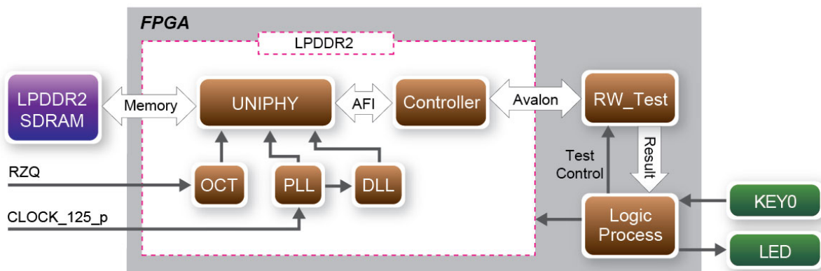
Figure 5-1 Block Diagram of the LPDDR2 SDRAM (512MB) Demonstration
