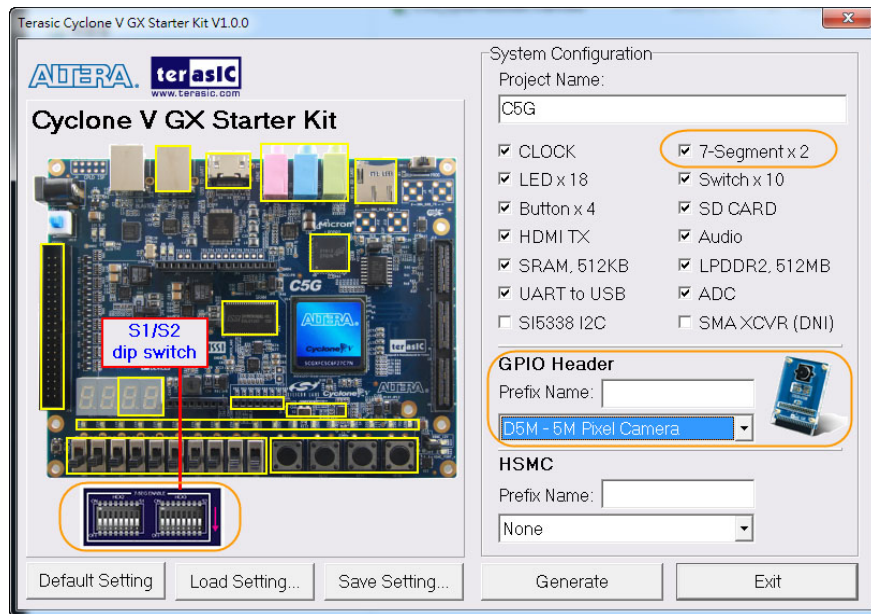
Figure 4-5 GPIO Expansion
