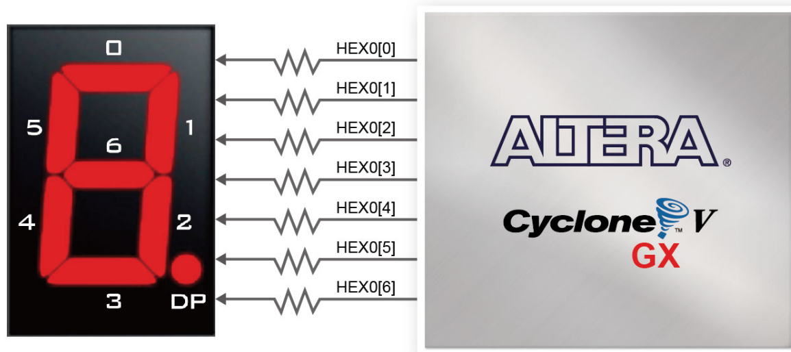
Figure 3-12 Connections between the 7-segment display HEX0 and Cyclone V GX FPGA
