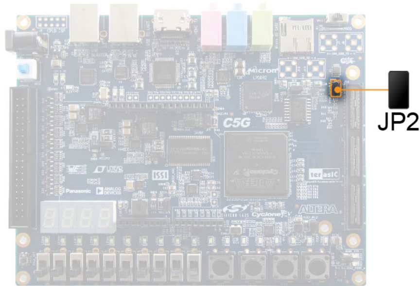
Figure 3-2 The JTAG chain configuration header
