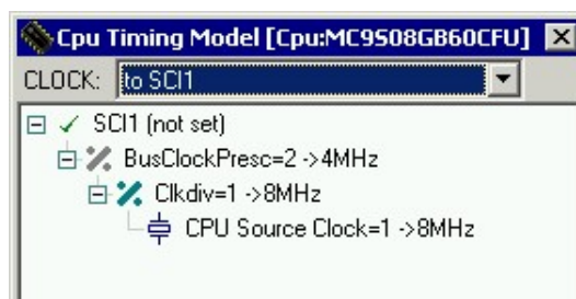
Figure 2.38 - CPU Timing Of Selected Peripheral
