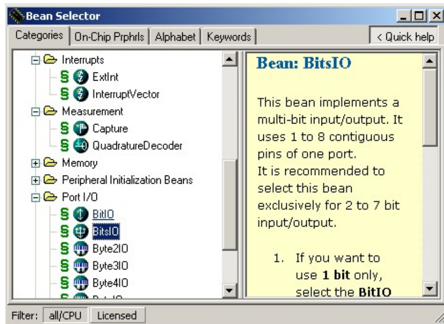
Figure 2.7 - Bean Selector with Quick Help panel
