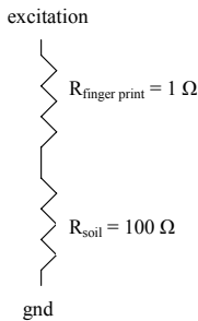
Figure 3a: Simplified circuit of contaminated probe in low EC (high resistance) soil. R_{\text{total}} = 101 \Omega , fingerprint causes 1% error.
