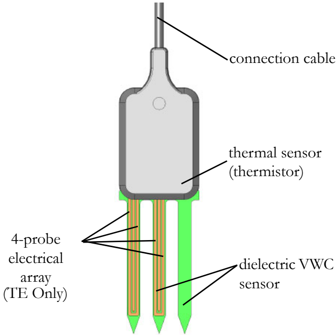
Figure 1: ECH 2 O-TE/EC-TM components
