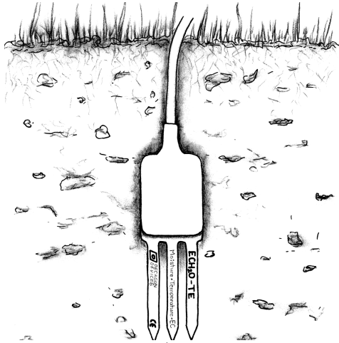
Figure 2: ECH 2 O-TE/EC-TM installed correctly
