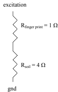
Figure 3b: Simplified circuit of contaminated probe in high EC (low resistance) soil. R_{\text{total}} = 5 \Omega , fingerprint causes 25% error
