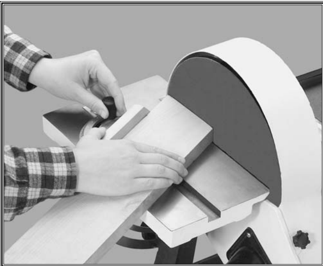
Figure 36. Using miter gauge to sand angles.
