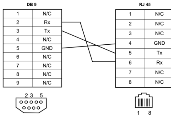
Figure 3. Console pinout
